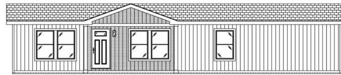
FRONT SIDEWALL W/ STANDARD NOMINAL 16'-0" DORMER
