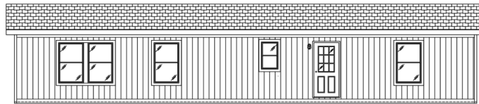
REAR SIDEWALL
