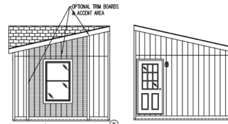
OPTIONAL FRONT ENDWALL WITH TRIM AND ACCENT AREA OPTIONAL DOOR ON FRONT ENDWALL
